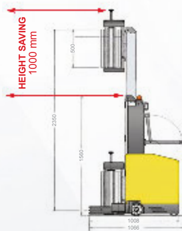
TELESCOPIC MAST
